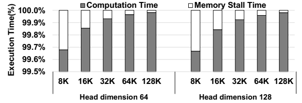
Figure 13. Computation time and memory stall time breakdown of AttenIO.
