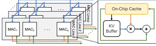
Figure 8. Organization of the PE array.
