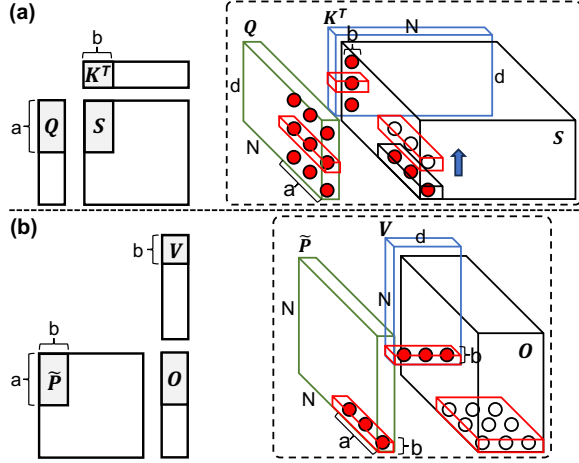
Figure 5. I/O-optimal CDAGs for long-sequence attention (a) computation of attention scores (S) with immediate reuse of partial results, and (b) computation of outputs (O).
